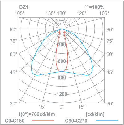
Optic C for escape route
